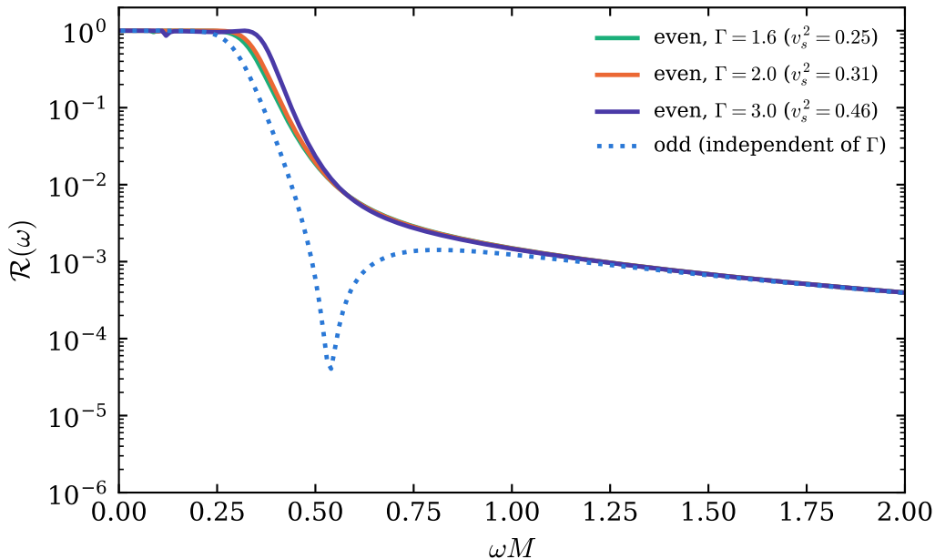
Even parity, R = 3M , \ell = 2 : dependence on the equation of state
